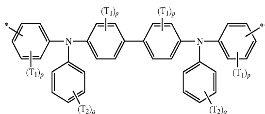
Formula 3l
