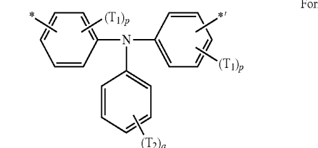
Formula 3l
