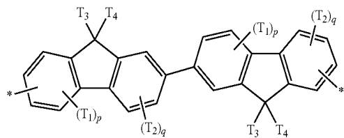
Formula 3f
