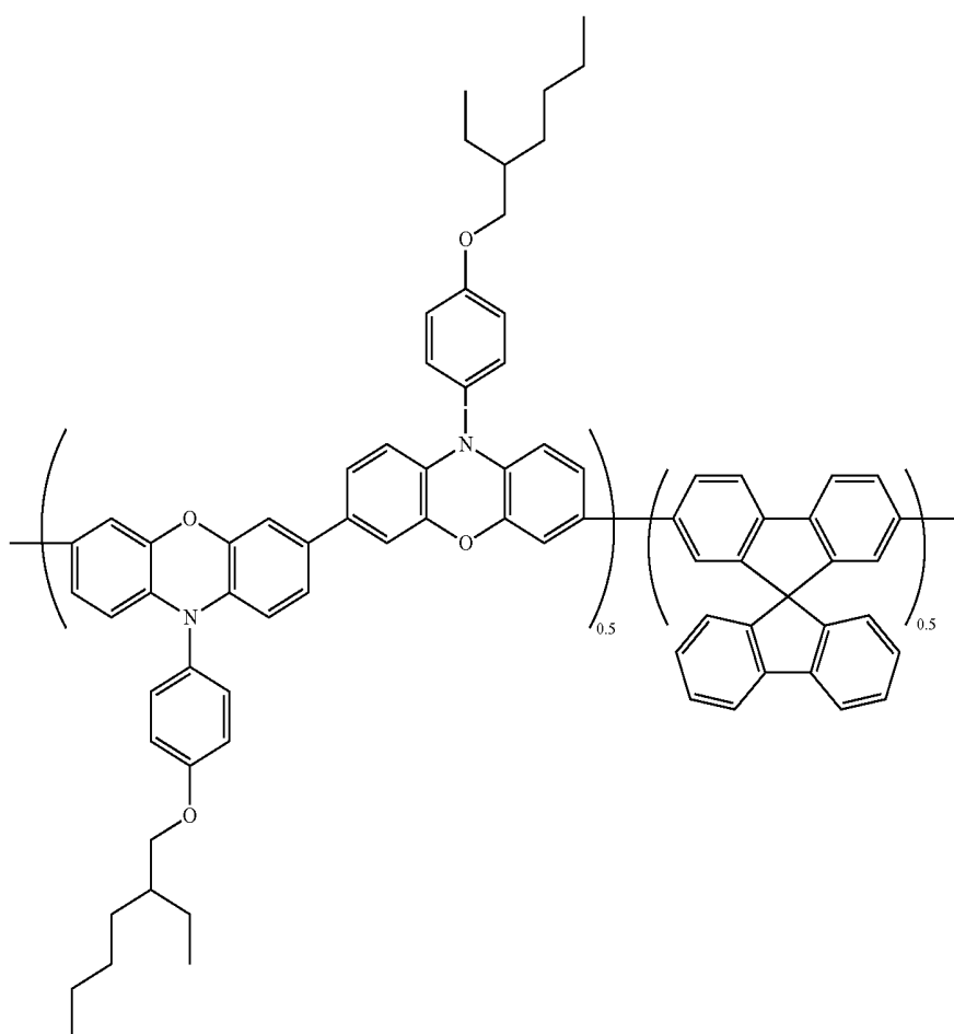
Polymer 2
