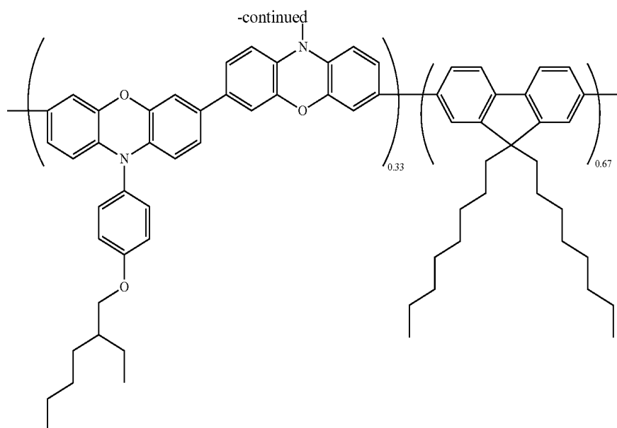
Polymer 3
