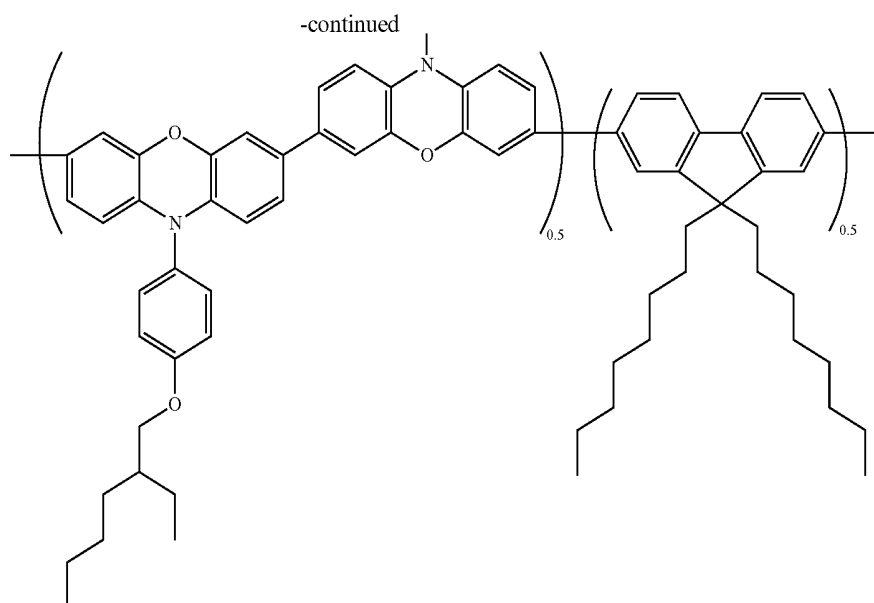
Polymer 1
