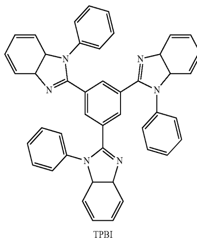
TPBI
