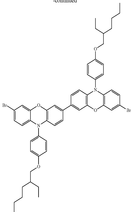
Compound (e)
