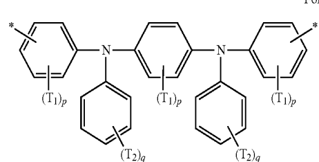
Formula 3k
